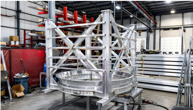
Welded aluminum structural frame at FWM.
